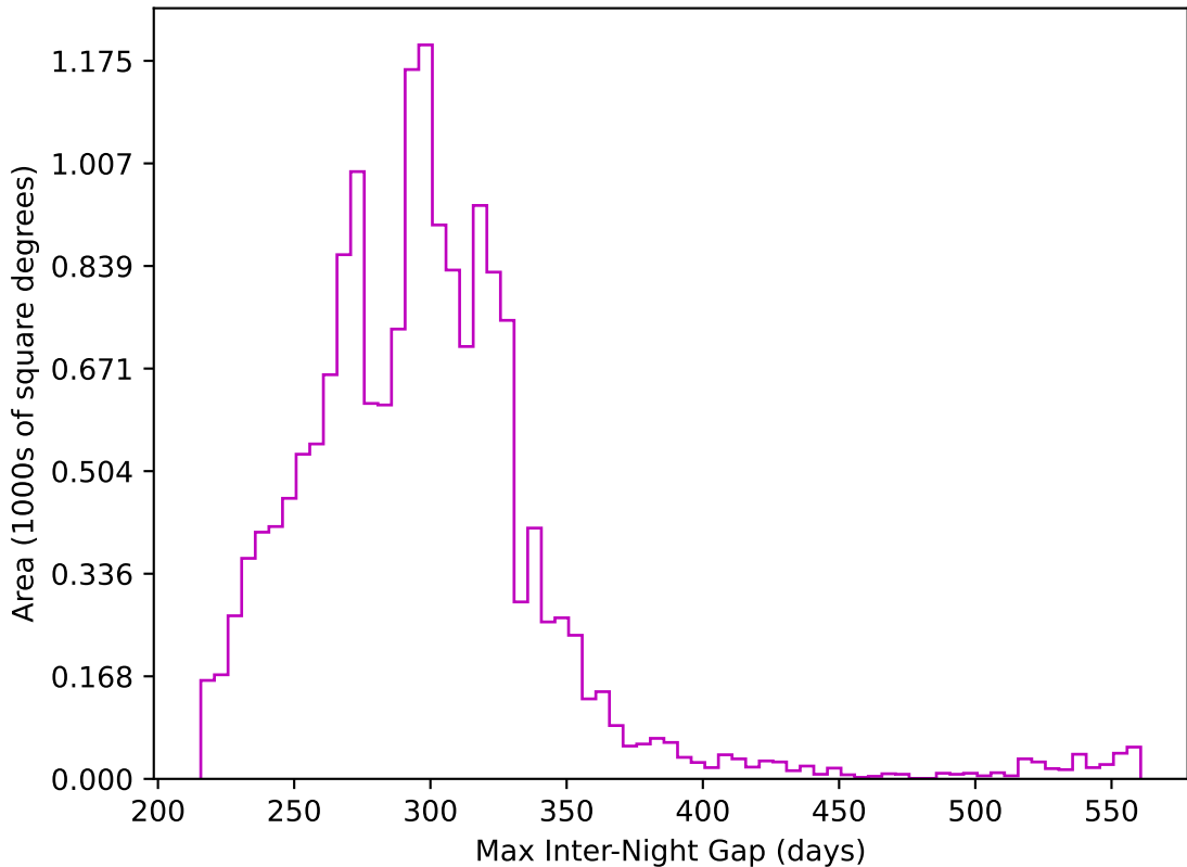
ddf_acor_sf15_lsf30_lsr20_v3.4_10yrs WFD z band: Max Inter-Night Gap
