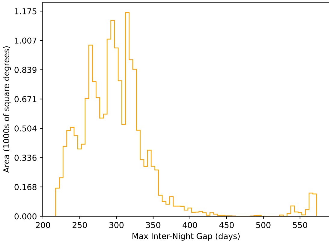
ddf_acor_sf15_lsf30_lsr20_v3.4_10yrs WFD r band: Max Inter-Night Gap
