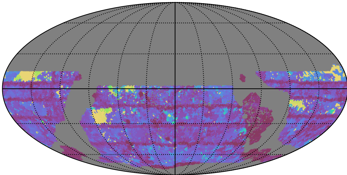
ddf_acor_sf15_lsf30_lsr20_v3.4_10yrs WFD i band: Max Inter-Night Gap
