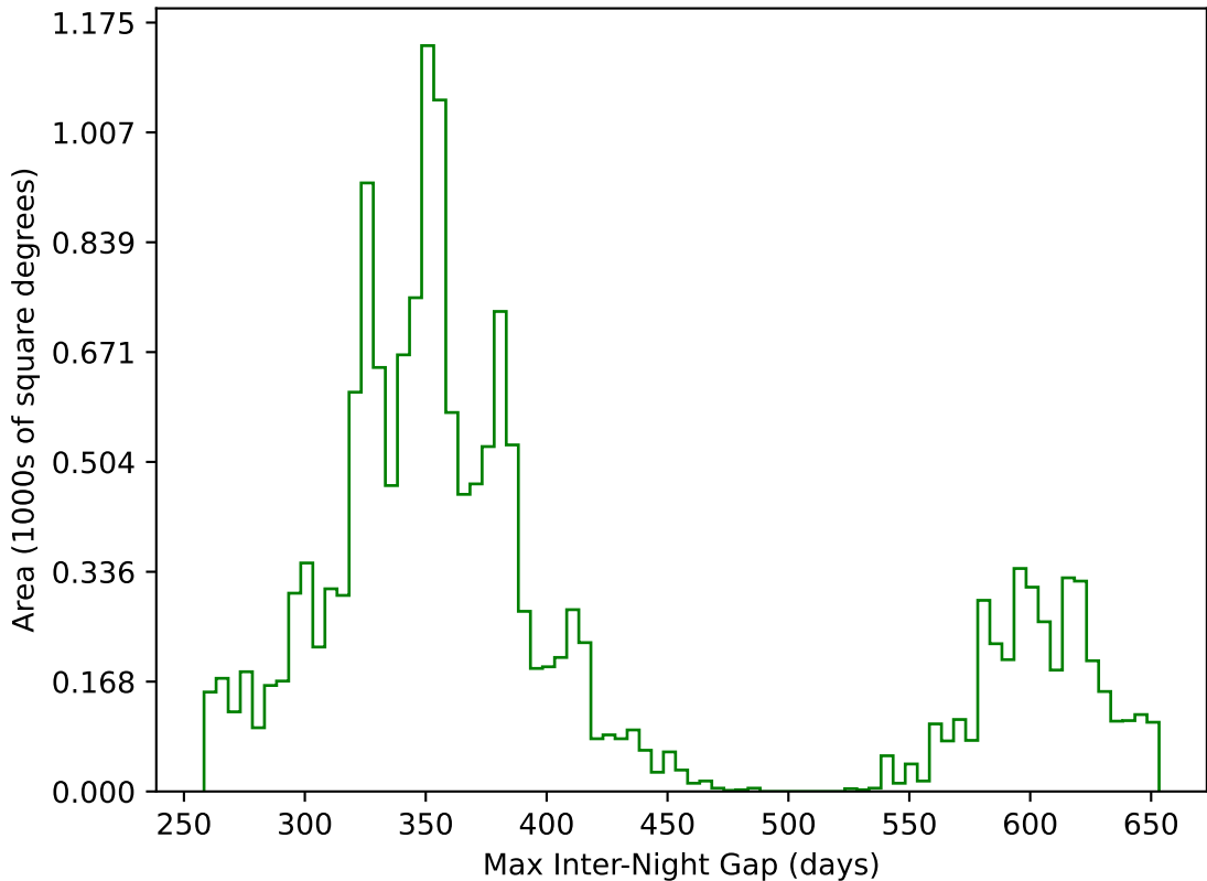
ddf_acor_sf15_lsf30_lsr20_v3.4_10yrs WFD g band: Max Inter-Night Gap
