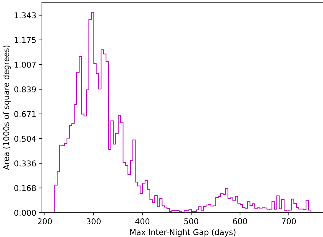
ddf_acor_sf15_lsf30_lsr20_v3.4_10yrs All sky z band: Max Inter-Night Gap
