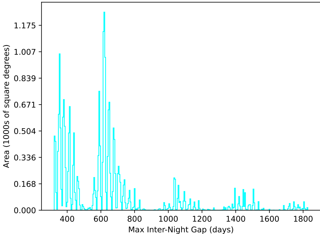
ddf_acor_sf15_lsf30_lsr20_v3.4_10yrs All sky u band: Max Inter-Night Gap
