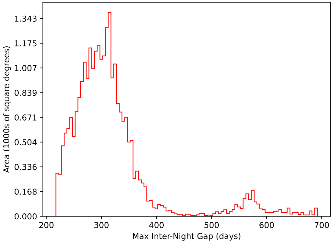
ddf_acor_sf15_lsf30_lsr20_v3.4_10yrs All sky i band: Max Inter-Night Gap
