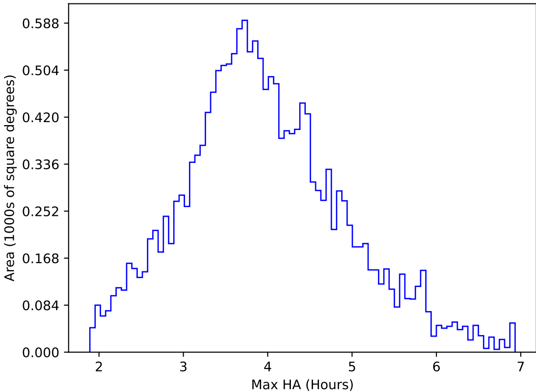
ddf_acor_sf15_lsf30_lsr20_v3.4_10yrs WFD u band: Max HA
