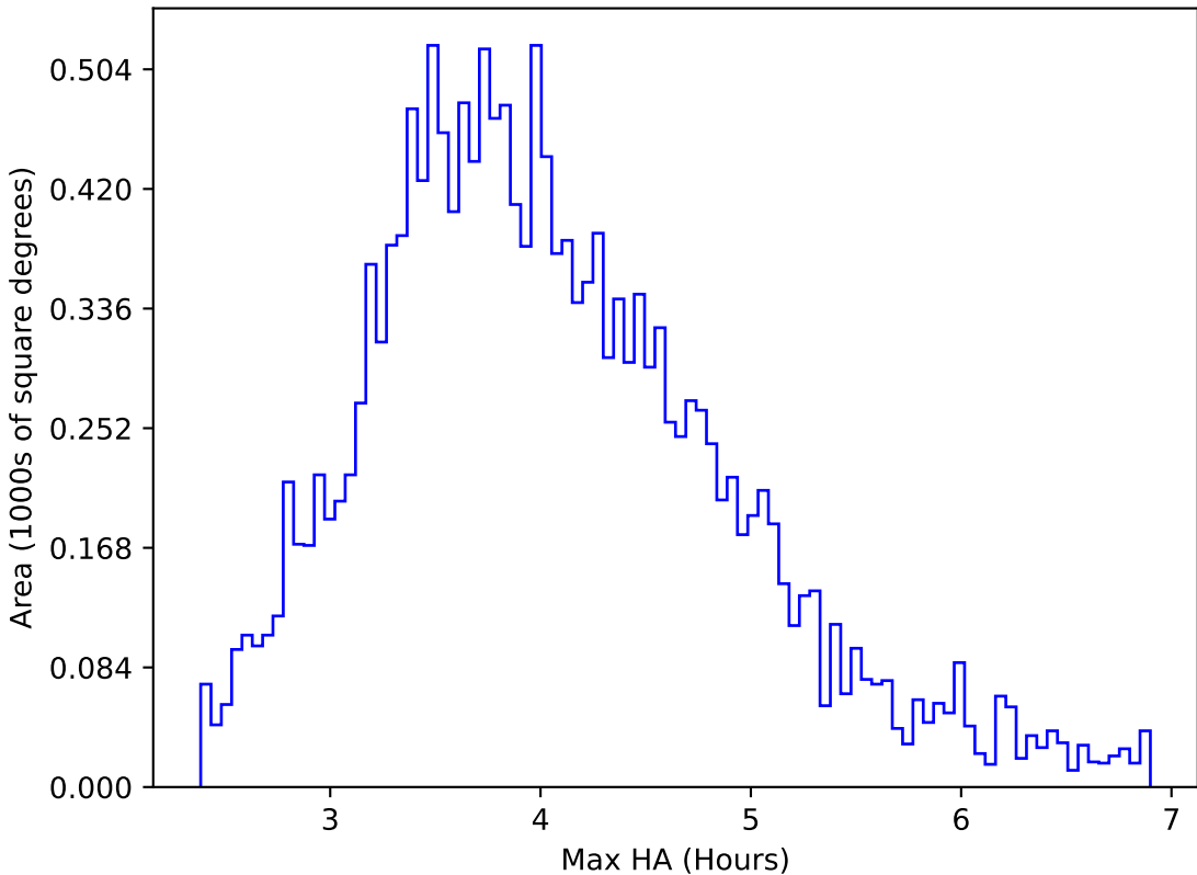
ddf_acor_sf15_lsf30_lsr20_v3.4_10yrs WFD g band: Max HA
