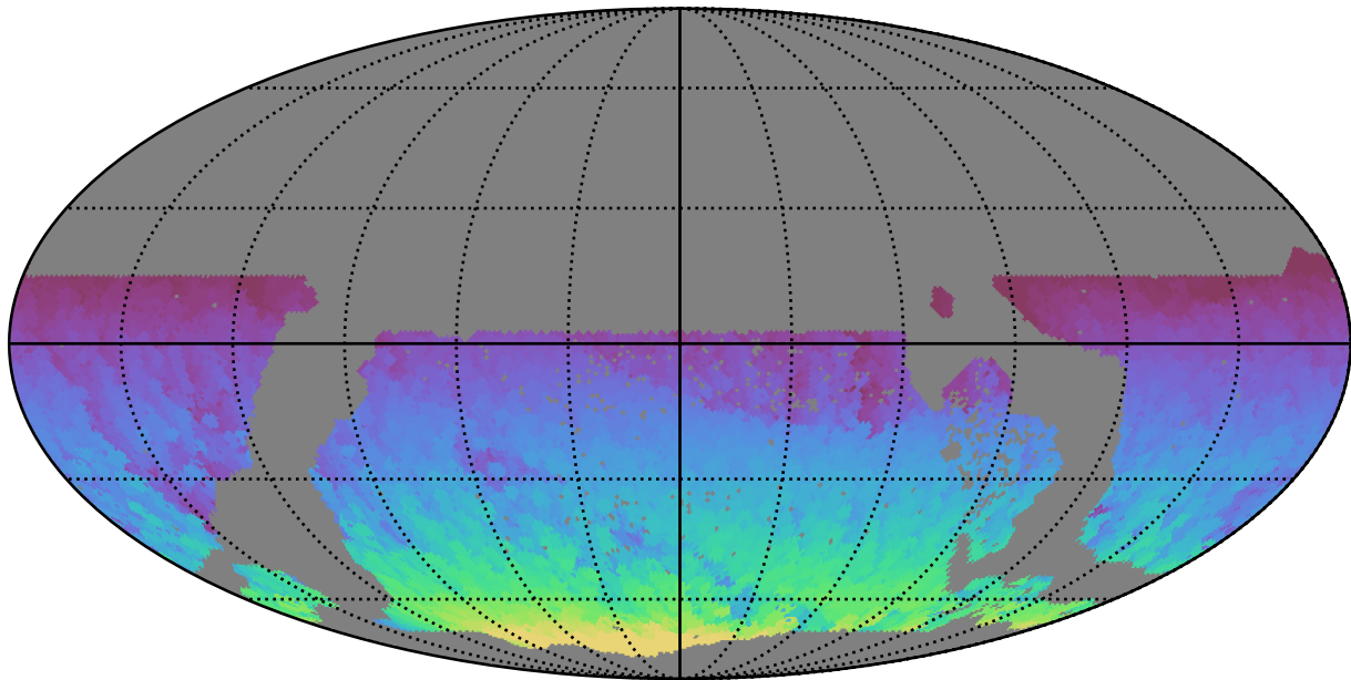
ddf_acor_sf15_lsf30_lsr20_v3.4_10yrs WFD all bands: Max HA
