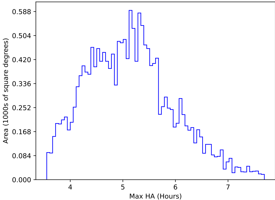
ddf_acor_sf15_lsf30_lsr20_v3.4_10yrs WFD all bands: Max HA
