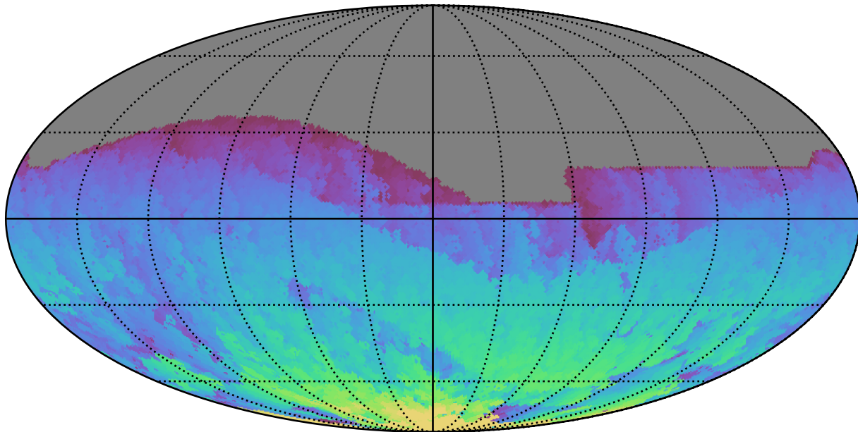
ddf_acor_sf15_lsf30_lsr20_v3.4_10yrs All sky z band: Max HA
