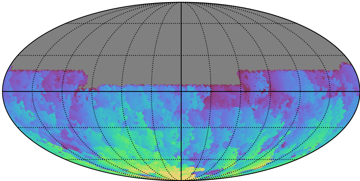
ddf_acor_sf15_lsf30_lsr20_v3.4_10yrs All sky u band: Max HA
