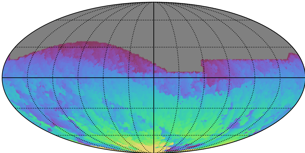
ddf_acor_sf15_lsf30_lsr20_v3.4_10yrs All sky i band: Max HA
