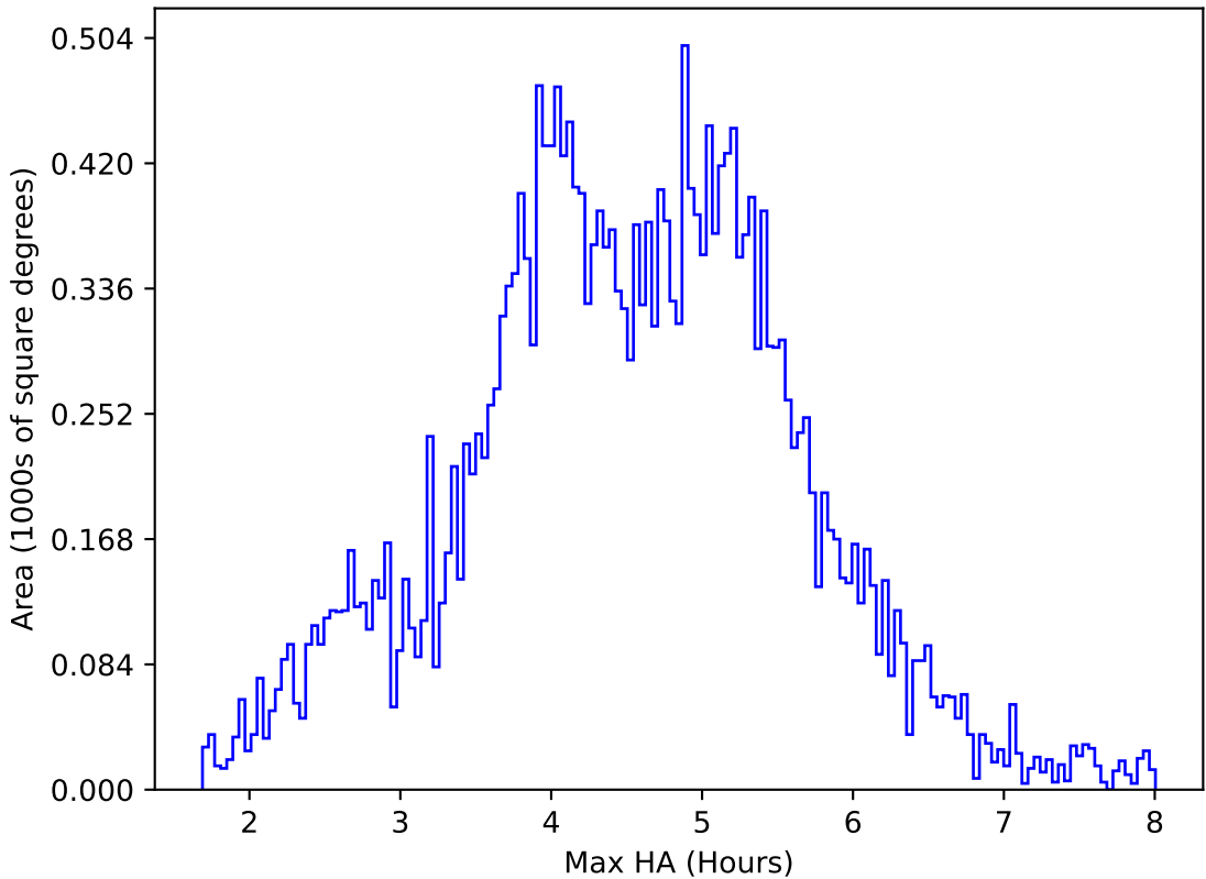
ddf_acor_sf15_lsf30_lsr20_v3.4_10yrs All sky i band: Max HA
