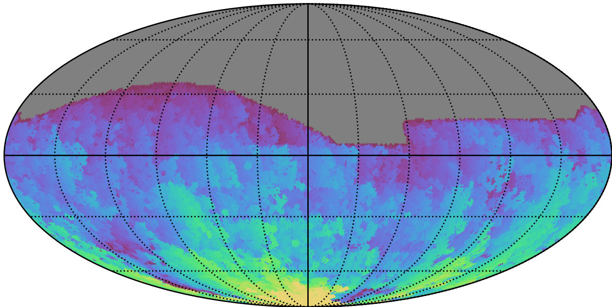
ddf_acor_sf15_lsf30_lsr20_v3.4_10yrs All sky g band: Max HA
