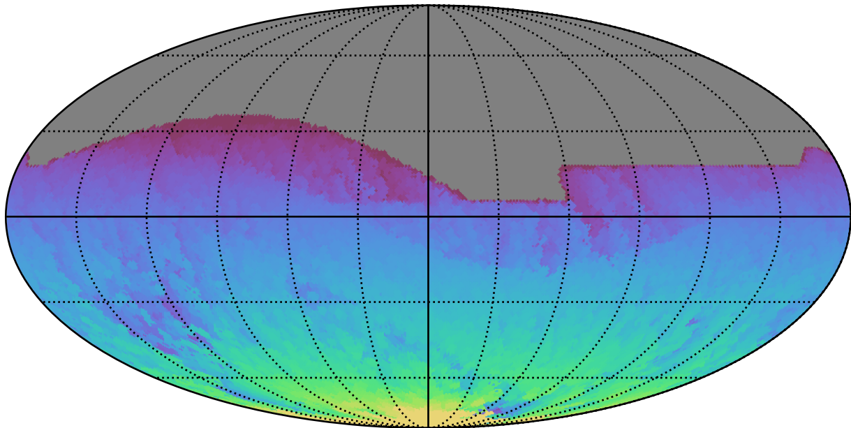
ddf_acor_sf15_lsf30_lsr20_v3.4_10yrs All sky all bands: Max HA
