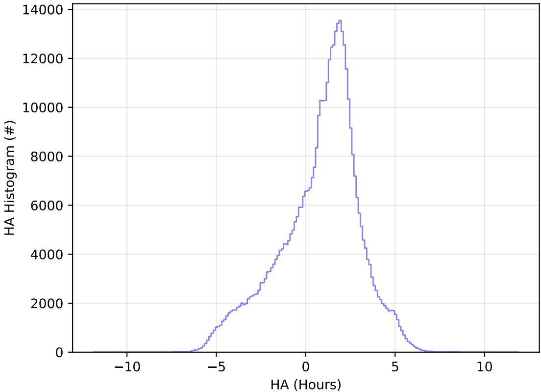
ddf_acor_sf15_lsf30_lsr20_v3.4_10yrs WFD z band: HA Histogram
