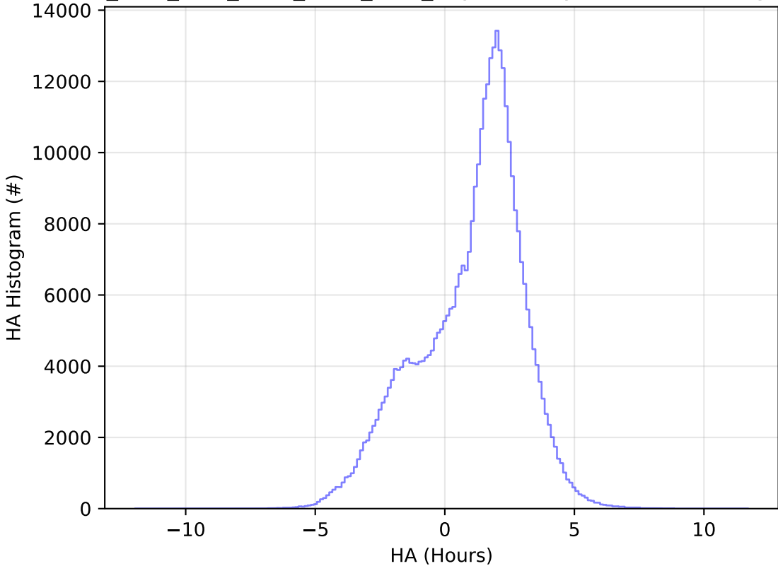
ddf_acor_sf15_lsf30_lsr20_v3.4_10yrs WFD y band: HA Histogram
