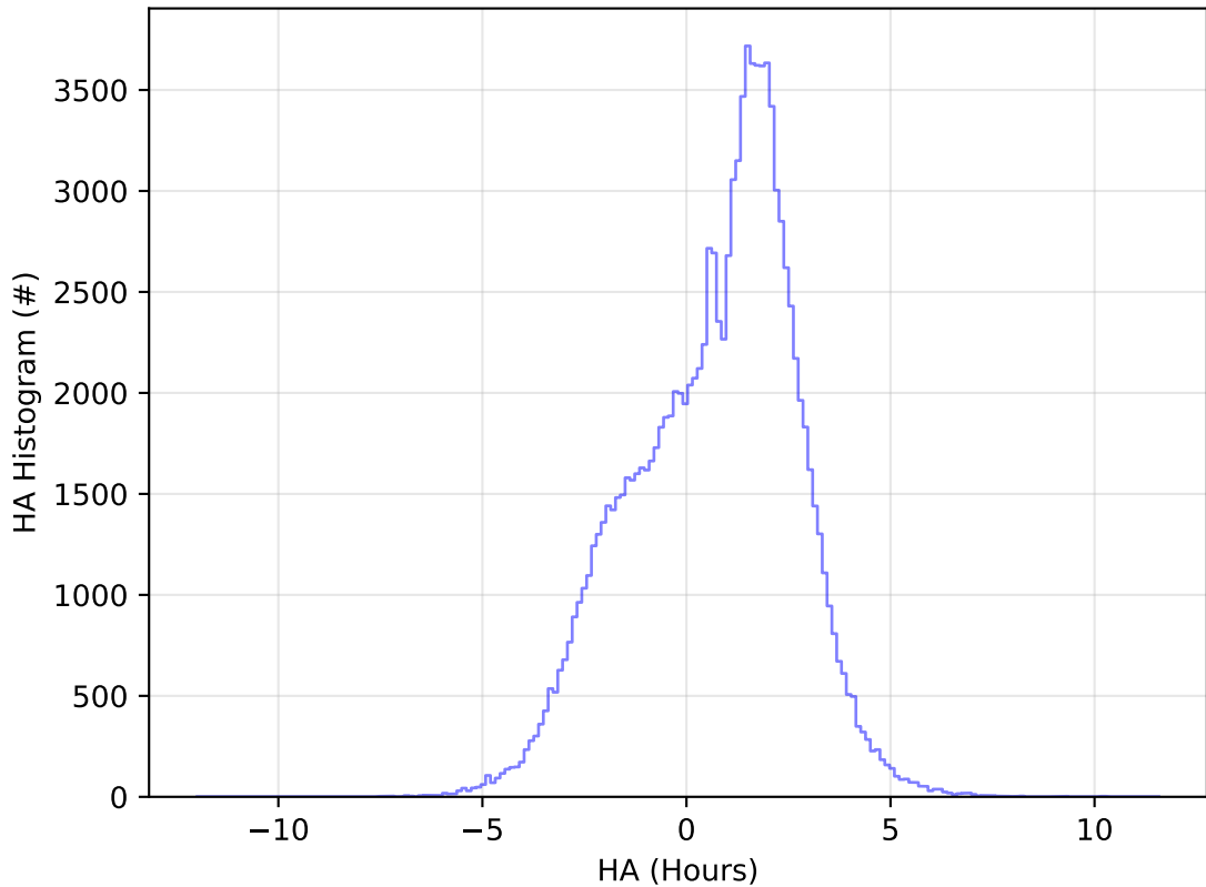
ddf_acor_sf15_lsf30_lsr20_v3.4_10yrs WFD u band: HA Histogram
