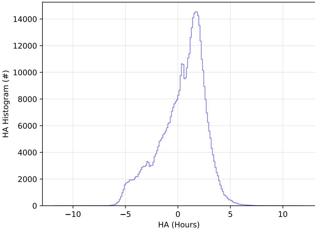
ddf_acor_sf15_lsf30_lsr20_v3.4_10yrs WFD r band: HA Histogram
