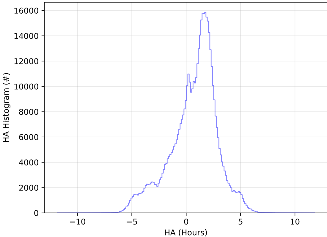
ddf_acor_sf15_lsf30_lsr20_v3.4_10yrs WFD i band: HA Histogram
