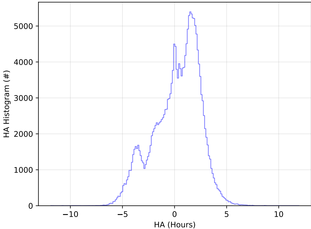
ddf_acor_sf15_lsf30_lsr20_v3.4_10yrs WFD g band: HA Histogram
