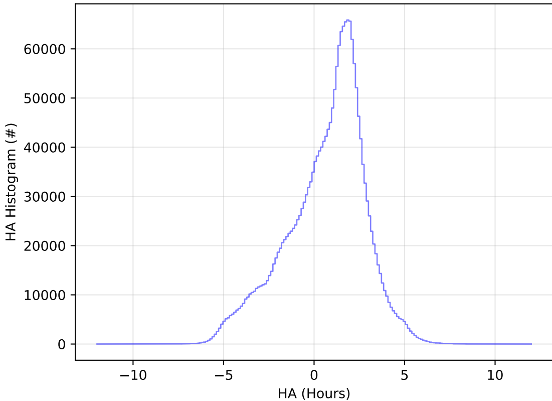
ddf_acor_sf15_lsf30_lsr20_v3.4_10yrs WFD all bands: HA Histogram
