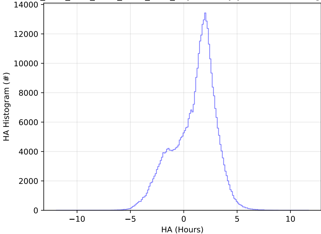
ddf_acor_sf15_lsf30_lsr20_v3.4_10yrs All sky y band: HA Histogram
