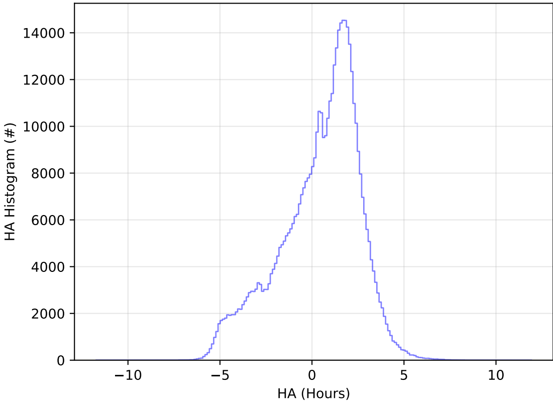
ddf_acor_sf15_lsf30_lsr20_v3.4_10yrs All sky r band: HA Histogram
