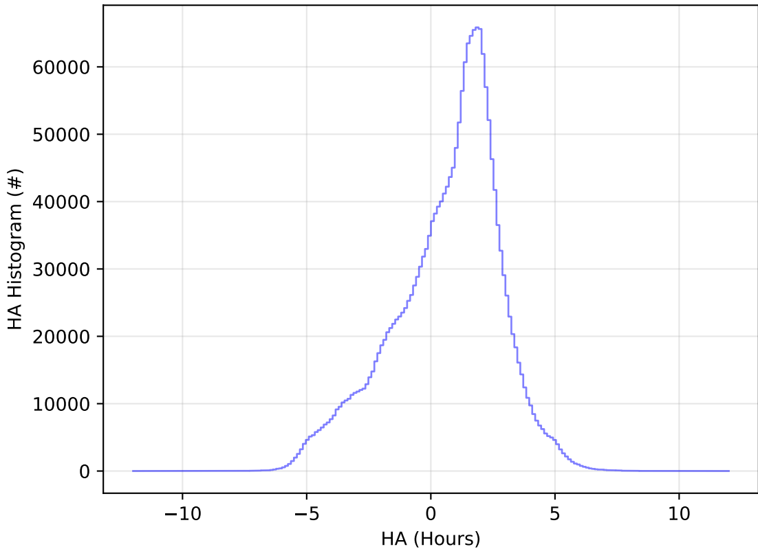
ddf_acor_sf15_lsf30_lsr20_v3.4_10yrs All sky all bands: HA Histogram
