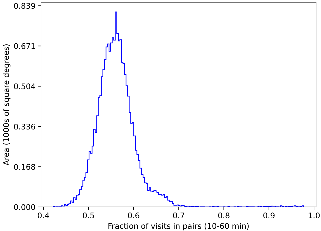
ddf_acor_sf15_lsf30_lsr20_v3.4_10yrs gri WFD: Fraction of visits in pairs (10-60 min)
