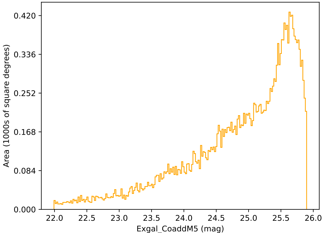
ddf_acor_sf15_lsf30_lsr20_v3.4_10yrs Yr 3-4 r band: Exgal_CoaddM5
