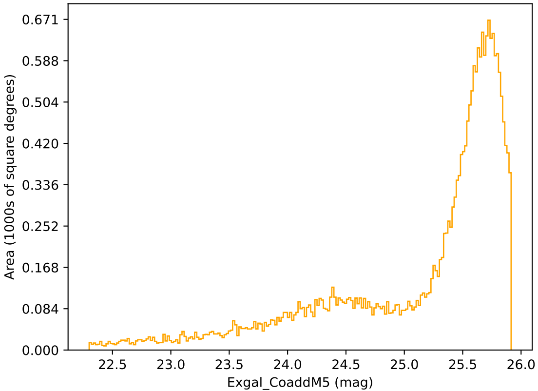
ddf_acor_sf15_lsf30_lsr20_v3.4_10yrs Yr 1 r band: Exgal_CoaddM5
