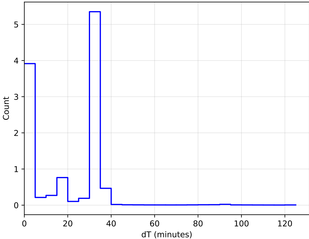
ddf_acor_sf15_lsf30_lsr20_v3.4_10yrs WFD: DeltaT Histogram 1e6
