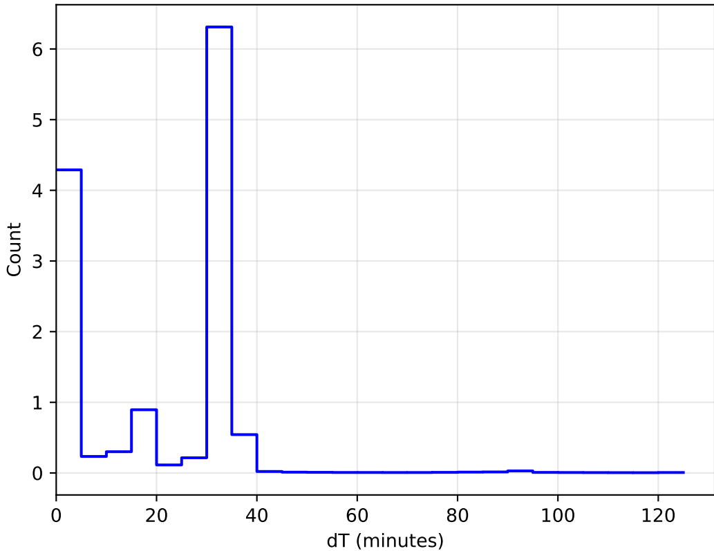
ddf_acor_sf15_lsf30_lsr20_v3.4_10yrs All sky: DeltaT Histogram
