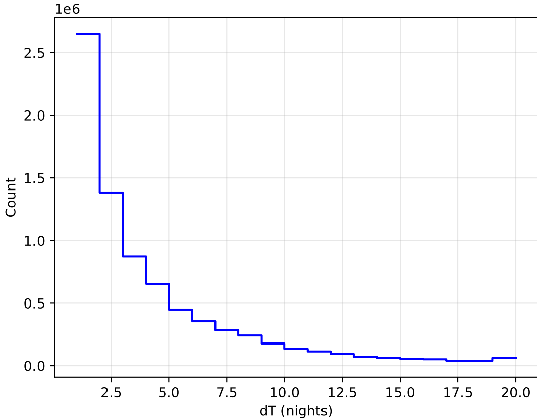
ddf_acor_sf15_lsf30_lsr20_v3.4_10yrs WFD all bands: DeltaNight Histogram
