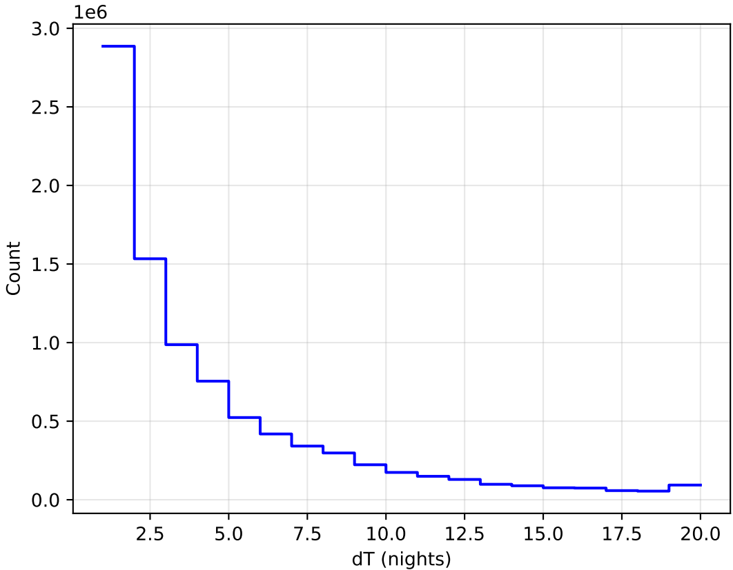
ddf_acor_sf15_lsf30_lsr20_v3.4_10yrs All sky all bands: DeltaNight Histogram
