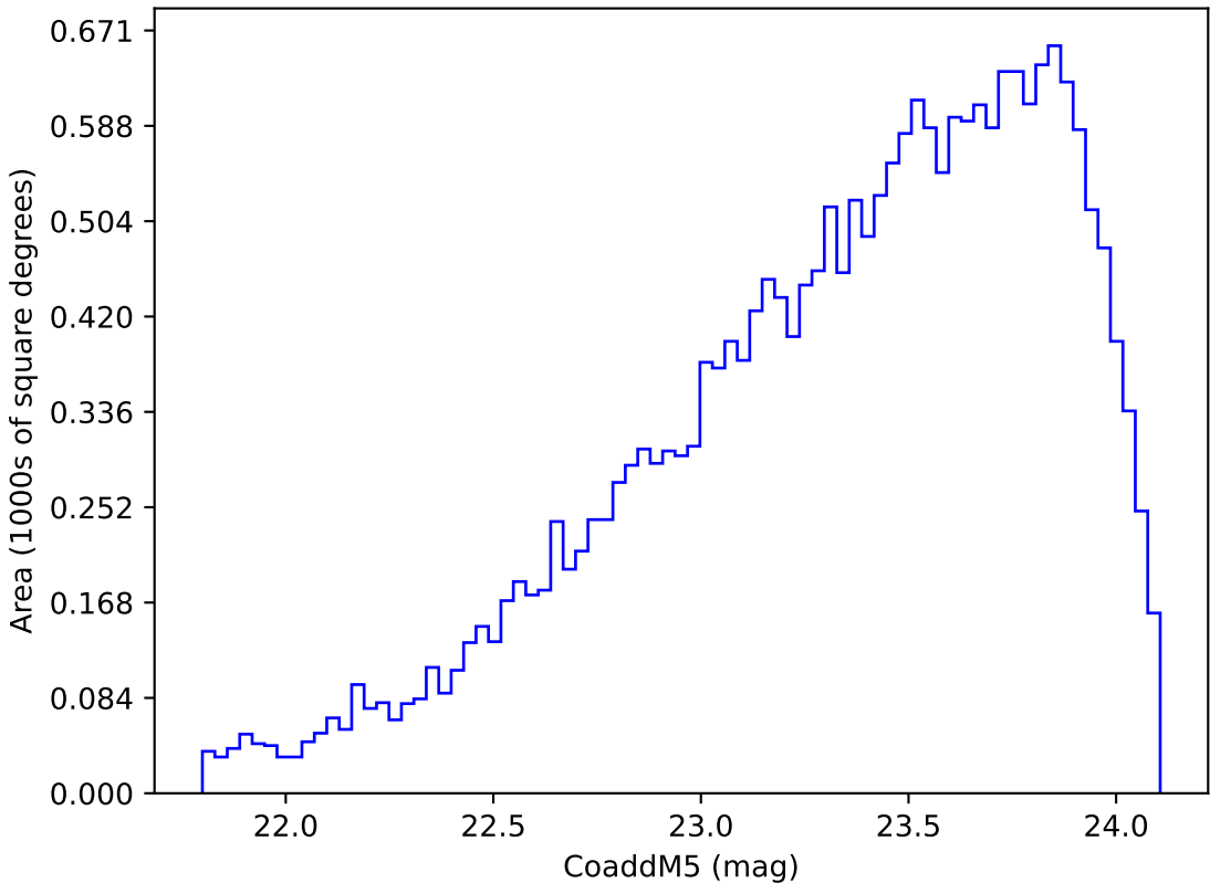
ddf_acor_sf15_lsf30_lsr20_v3.4_10yrs Yr 3-4 y band: CoaddM5
