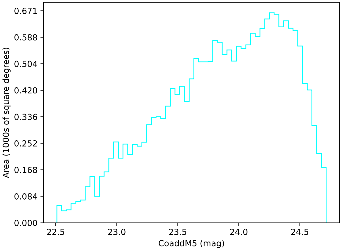
ddf_acor_sf15_lsf30_lsr20_v3.4_10yrs Yr 3-4 u band: CoaddM5
