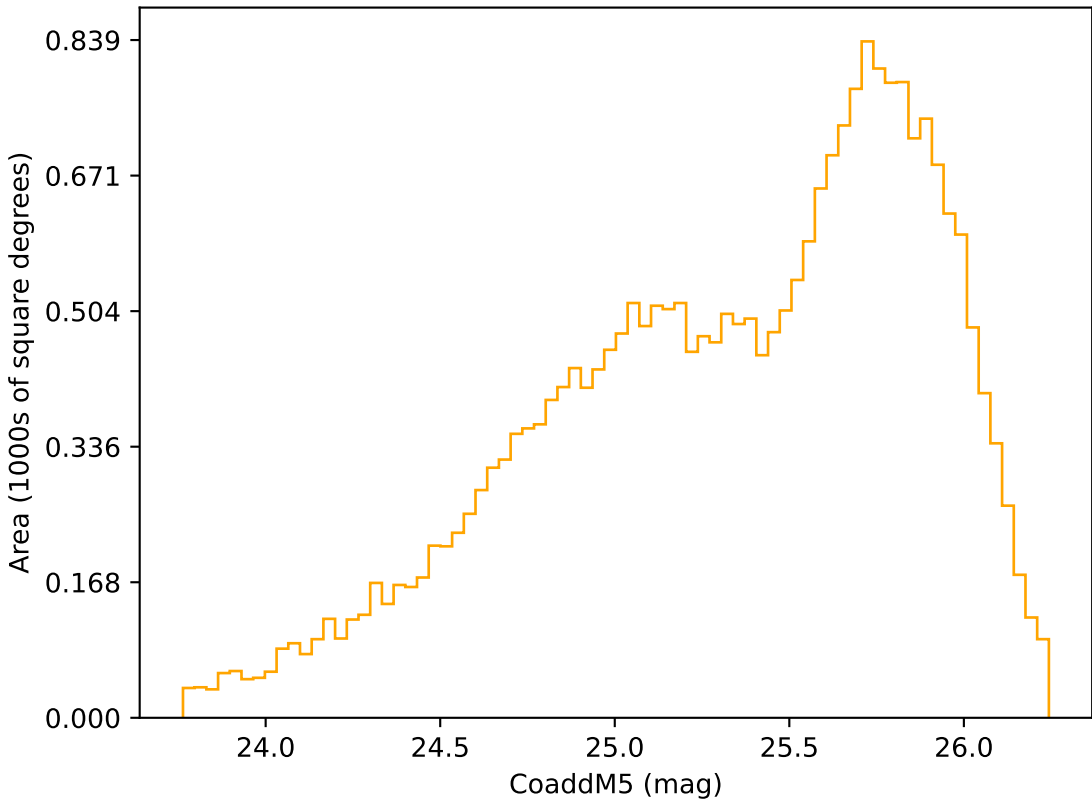
ddf_acor_sf15_lsf30_lsr20_v3.4_10yrs Yr 3-4 r band: CoaddM5
