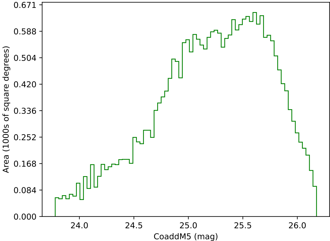
ddf_acor_sf15_lsf30_lsr20_v3.4_10yrs Yr 3-4 g band: CoaddM5
