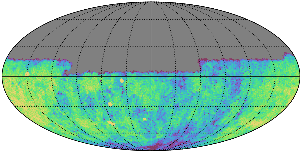
ddf_acor_sf15_lsf30_lsr20_v3.4_10yrs Yr 1 u band: CoaddM5
