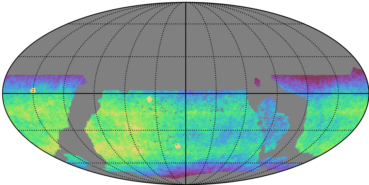
ddf_acor_sf15_lsf30_lsr20_v3.4_10yrs WFD z band: CoaddM5
