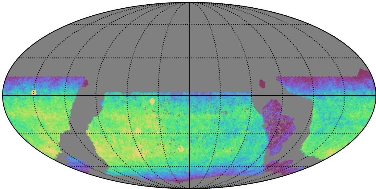
ddf_acor_sf15_lsf30_lsr20_v3.4_10yrs WFD y band: CoaddM5
