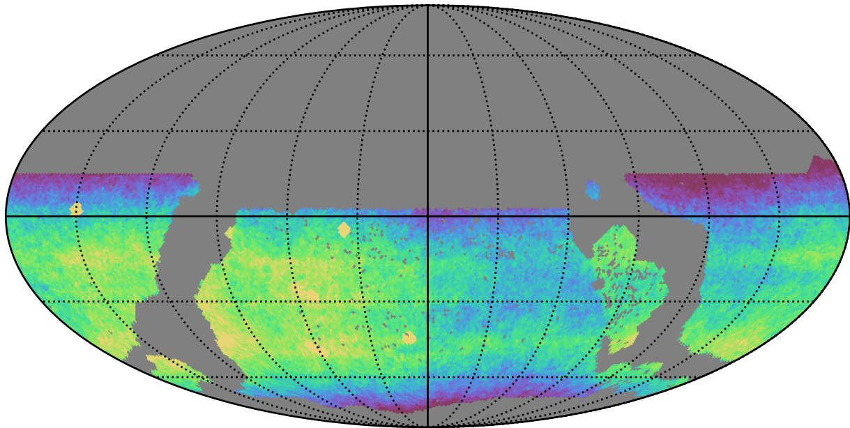
ddf_acor_sf15_lsf30_lsr20_v3.4_10yrs WFD r band: CoaddM5
