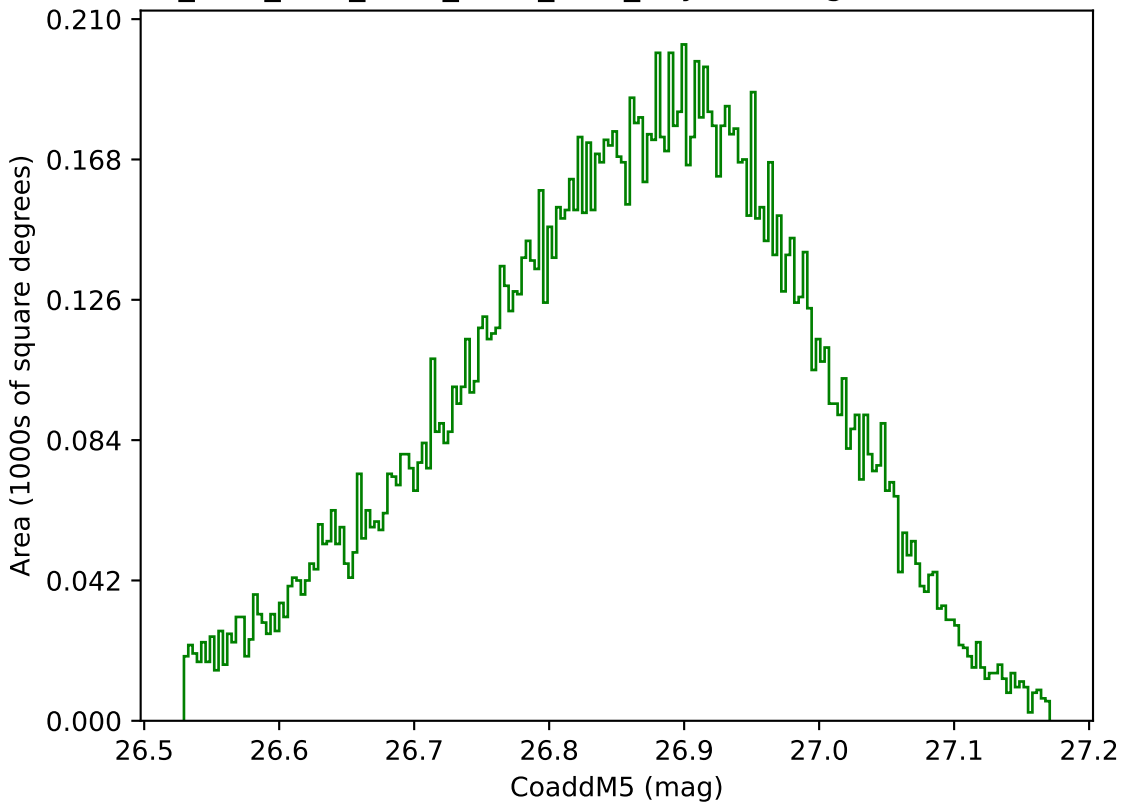
ddf_acor_sf15_lsf30_lsr20_v3.4_10yrs WFD g band: CoaddM5
