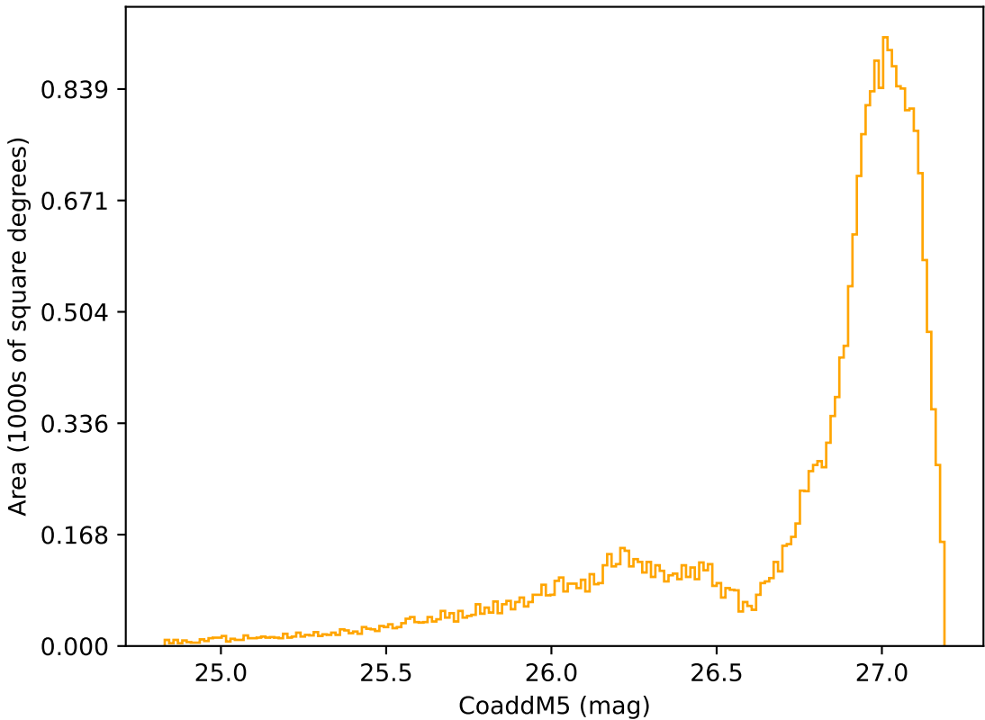
ddf_acor_sf15_lsf30_lsr20_v3.4_10yrs All sky r band: CoaddM5
