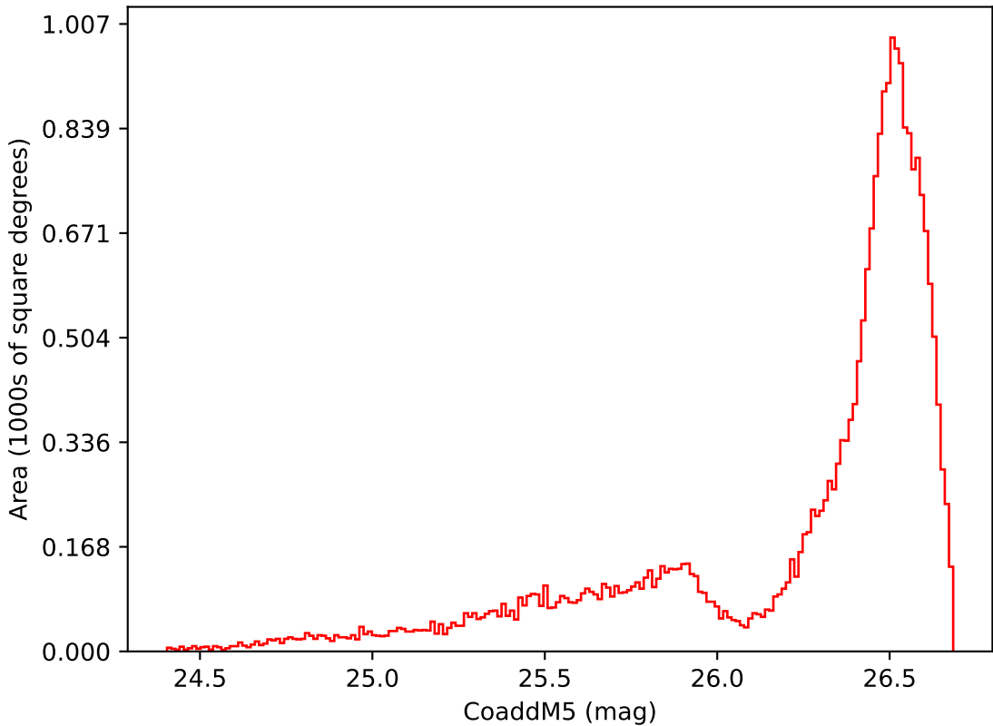
ddf_acor_sf15_lsf30_lsr20_v3.4_10yrs All sky i band: CoaddM5
