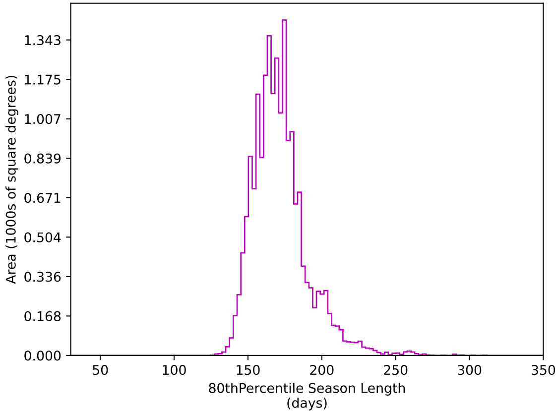
ddf_acor_sf15_lsf30_lsr20_v3.4_10yrs WFD z band: 80thPercentile Season Length
