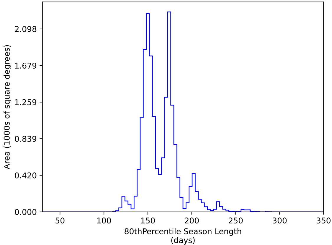
ddf_acor_sf15_lsf30_lsr20_v3.4_10yrs WFD y band: 80thPercentile Season Length
