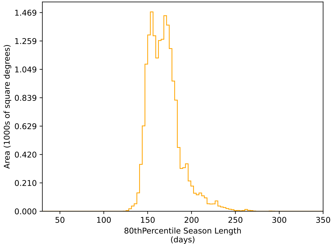
ddf_acor_sf15_lsf30_lsr20_v3.4_10yrs WFD r band: 80thPercentile Season Length
