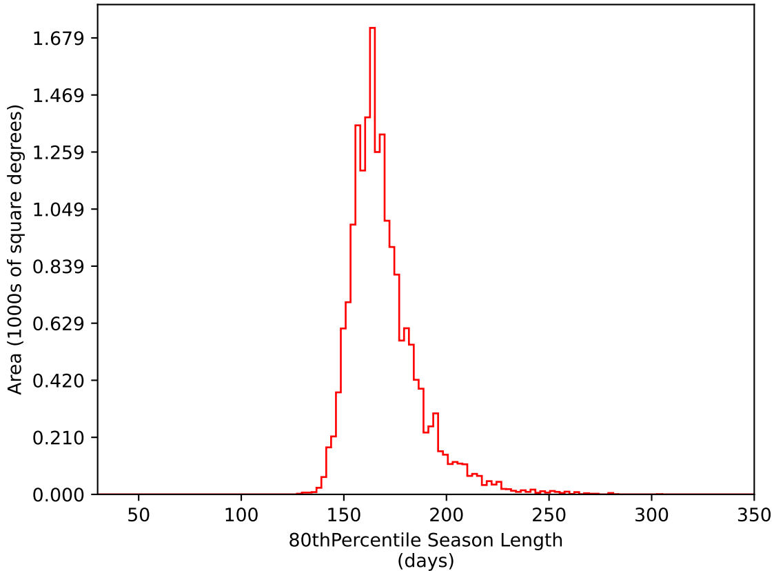
ddf_acor_sf15_lsf30_lsr20_v3.4_10yrs WFD i band: 80thPercentile Season Length
