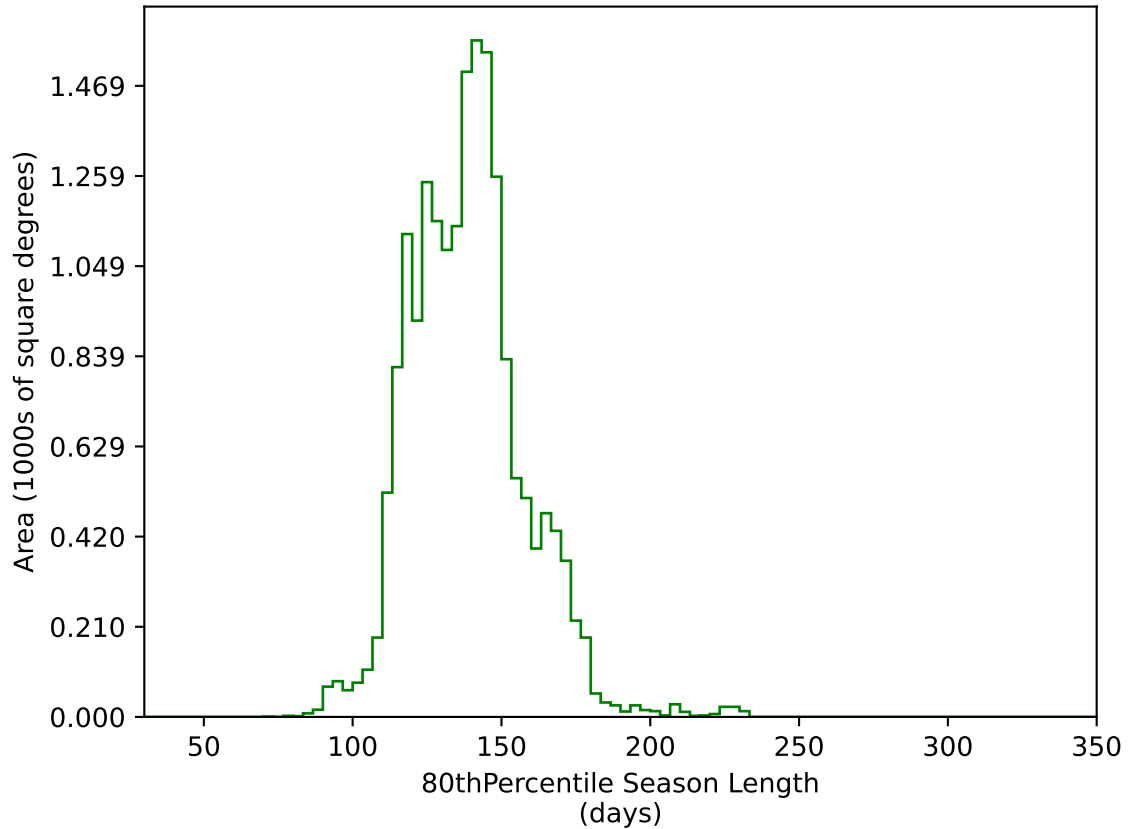
ddf_acor_sf15_lsf30_lsr20_v3.4_10yrs WFD g band: 80thPercentile Season Length
